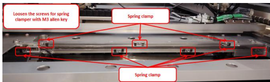
Figure 4: Y-Axis Quantic Scale
