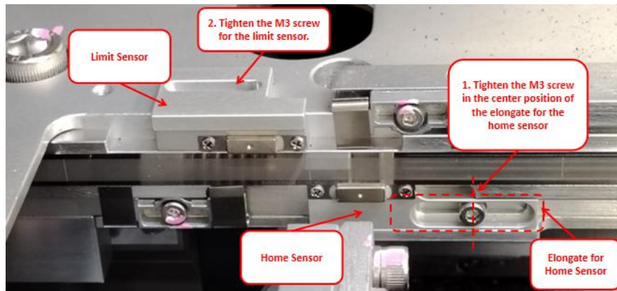
Figure 10: Y-Axis Home and Limit Sensors Alignment
