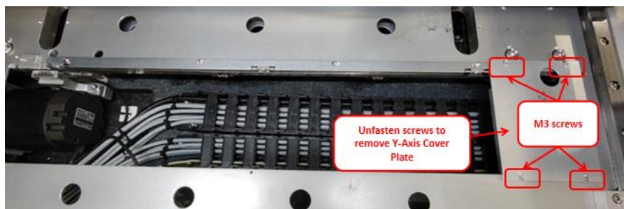
Figure 3: Y-Axis Cover Plate
