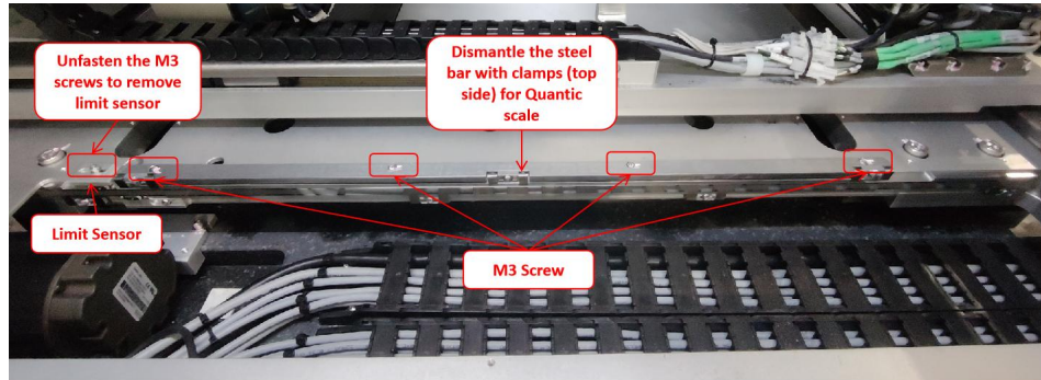
Figure 5: Y-Axis Mount Bar with Clamp (Top Side) & Limit Sensor
