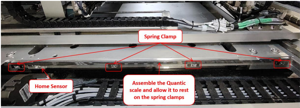
Figure 8: Y-Axis Quantic Scale (Sample Image)
