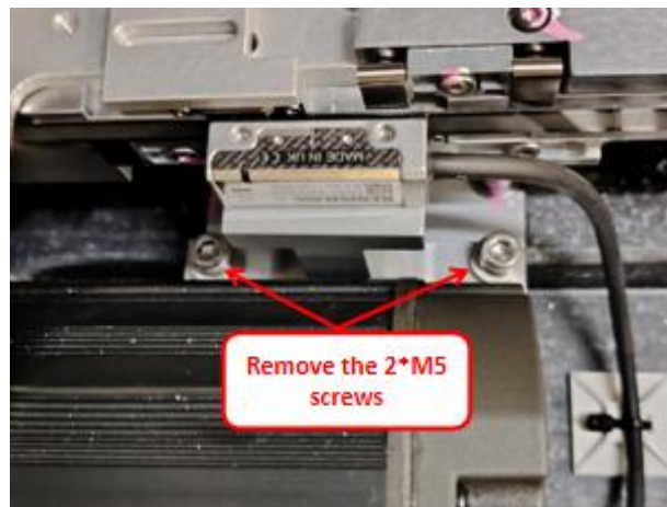
Figure 6: Y-Axis Encoder Bracket
